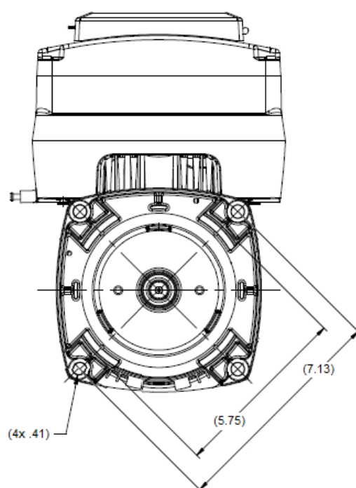
Shaft View
